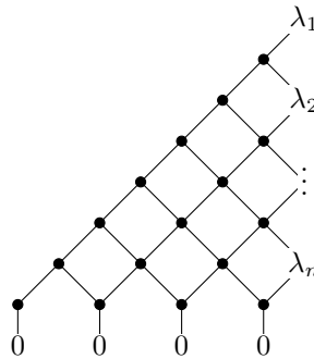
Figure 6: Marked Hasse diagram for \mathfrak{sp}_{2n} and \mathfrak{o}_{2n+1} .
