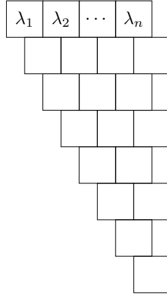
Figure 5: Board defining generalized Gelfand–Tsetlin patterns for \mathfrak{sp}_{2n} and \mathfrak{o}_{2n+1} .
