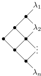
Figure 4: Marked Hasse diagram for \mathfrak{sl}_n .
