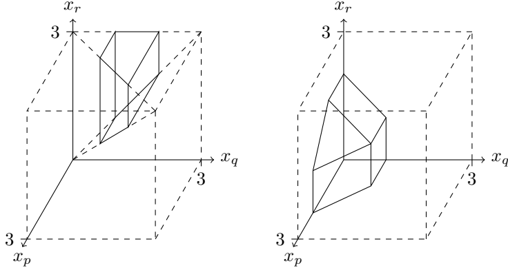
Figure 3: The marked order polytope of the marked poset in Figure 2 is given by the inequalities 0 \leq x_p \leq x_q \leq x_r \leq 3 and 1 \leq x_q \leq 2 . The marked chain polytope is given by the inequalities x_p, x_q, x_r \geq 0 , x_p + x_q + x_r \leq 3 , x_p + x_q \leq 2 , x_q + x_r \leq 2 , and x_q \leq 1 . Note that they are not combinatorially isomorphic.
