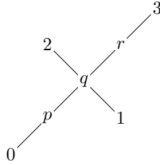
Figure 2: A marked Hasse diagram defining a partial order on the set P = \{p, q, r\} \cup A with |A| = 4 and \lambda = (3, 2, 1, 0) \in \mathbf{R}^A .
