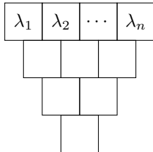
Figure 1: Board defining Gelfand–Tsetlin patterns.
