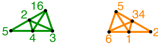
Figure 3: The point configuration A \subset \mathbb{P}^{r-1} = \mathbb{P}^2 and a dual configuration A^* \subset \mathbb{P}^{n-r-1} = \mathbb{P}^2 .
