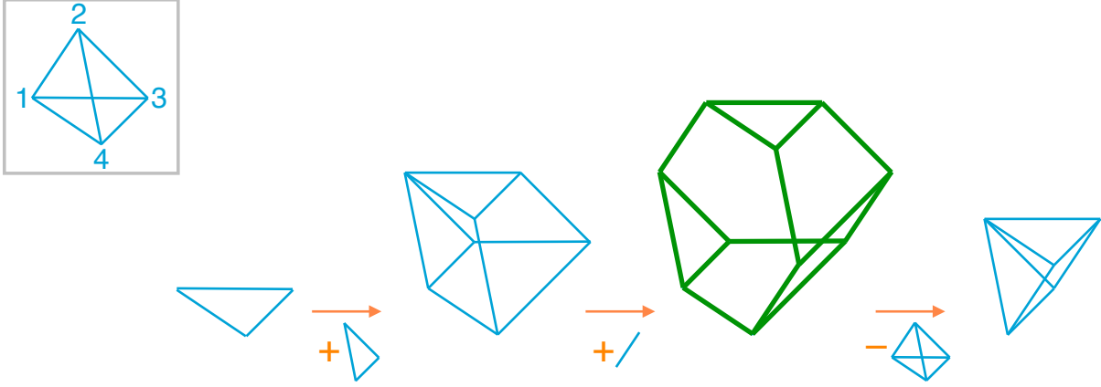
Figure 4: Building up the Minkowski sum \Delta_{134} + \Delta_{234} + \Delta_{12} = O_M and the signed Minkowski sum \Delta_{134} + \Delta_{234} + \Delta_{12} - \Delta_{1234} = P_M one step at a time.
