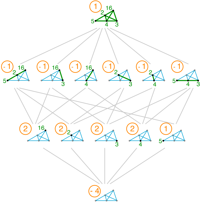
Figure 2: The Möbius function \mu(F, \hat{1}) of the lattice of flats M encodes the non-zero multigraded Betti numbers of I(\tilde{L}) .
