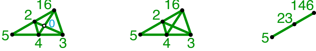
Figure 5: The triple (M_{hom}, M, M') corresponding to the affine subspace L .
