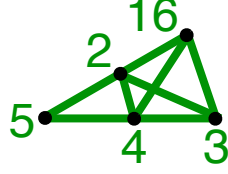
Figure 1: A point configuration A \subset \mathbb{P}^2 corresponding to the linear ideal I .
