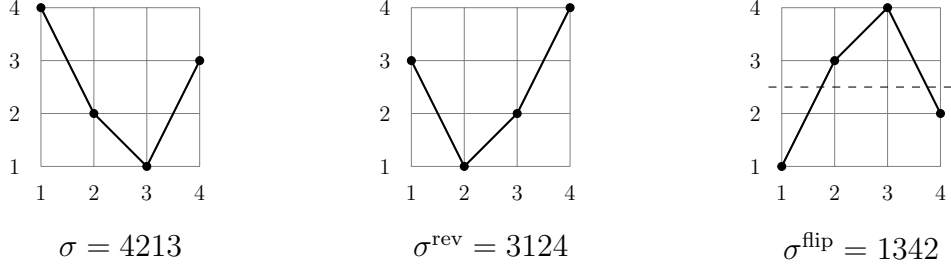
Figure 3.5: Permutation diagrams of \sigma , \sigma^{\text{rev}} and \sigma^{\text{flip}} respectively.
