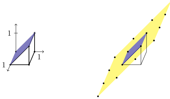
Figure 2.3: The relative volume of the blue facet of the 3-polytope is equal to 1.
