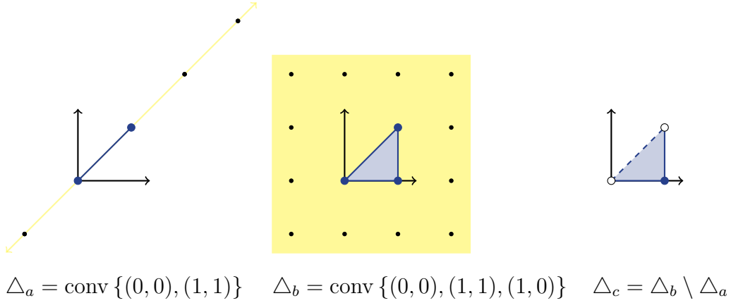
Figure 3.2: A unimodular 1-simplex, a unimodular 2-simplex and a half-open unimodular 2-simplex.
