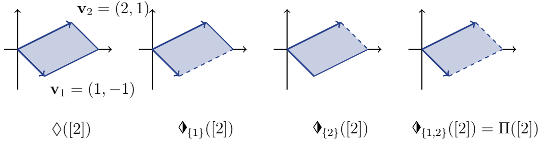
Figure 3.7: A closed 2-dimensional parallelepiped and its half-open variants.
