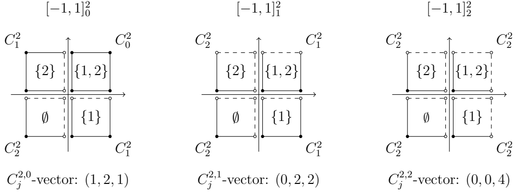
Figure 4.4: Decomposition of [-1, 1]_\ell^2 into unit cells indexed by subsets of \{1, 2\} for \ell = 0, 1, 2 .
