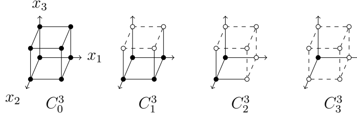
Figure 3.6: Half-open unit cubes C_j^3 for j = 0, 1, 2, 3 .
